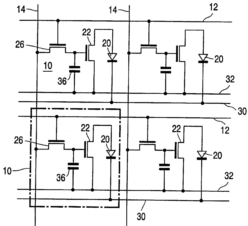
FIG. 2 PRIOR ART
